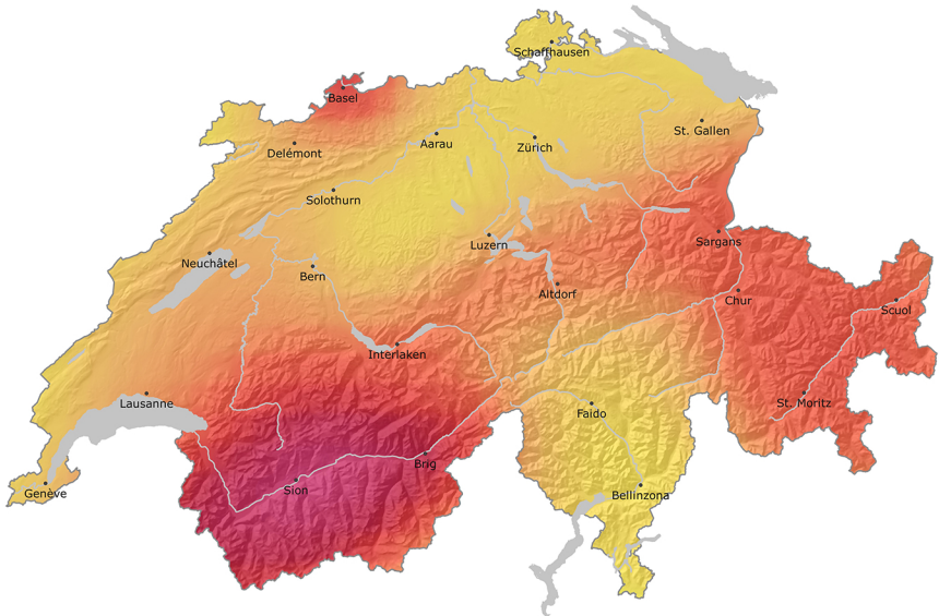
Seismic hazard horizontal acceleration at 5 hertz 10 % within fifty years
